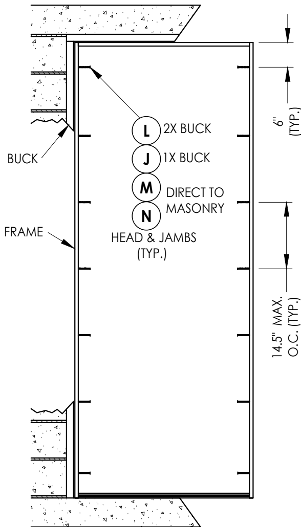
FRAME ANCHORING
